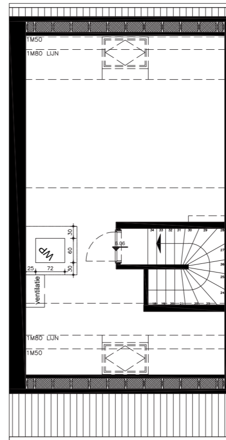
Zolder
